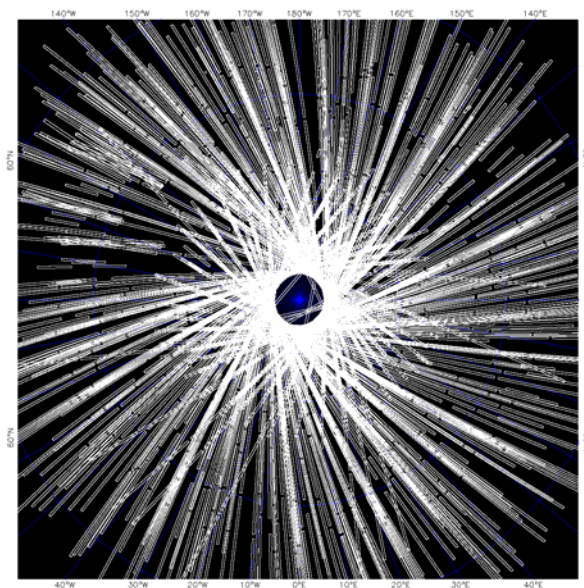
Figure 1. CRISM multispectral survey coverage of Mars Chart MC-01 ( >65^\circ N) through eight weeks of science operations. Vector outlines of \sim 1500 MSP strips are shown.
