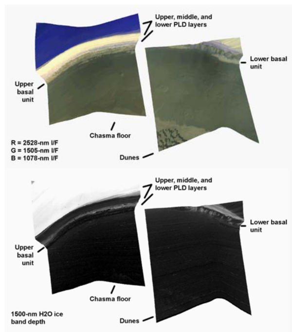
Figure 4. Atmospherically corrected, map projected CRISM targeted observations (2FA6; 3074) acquired near the head of Chasma Boreale. (top) IR false color composite (R:2.528, G:1.505, B:1.078 \mu\text{m} ); (bottom) 1.5 \mu\text{m} band depth (BD1500) spectral index. The three layer structure of the PLD is evident (ice rich upper surface; ice poor middle layer; ice-rich lower layer). The upper and lower basal units are dissimilar, but both are depleted in ice as compared to the PLD.
